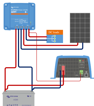
Solar charger system with inverter connected directly to the battery and controlled by the load output
