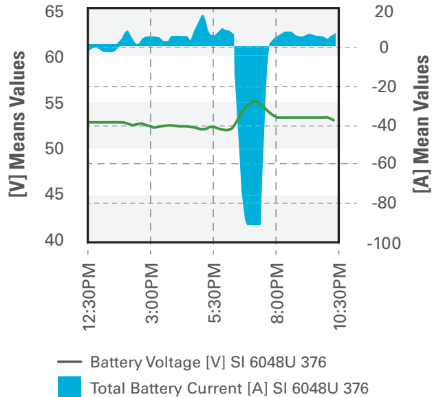
Graph 2. Charging cycle with Discover AES LiFePO 4 batteries. Almost the entire time that the generator was running at its maximum current. The runtime is just 1 hour instead of the 2.5 hours charging cycle with lead acid batteries. NOTE: The capacity being replaced (the load) in this 2017 analysis was approximately 20% larger than the load being replaced in 2016.
